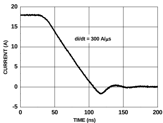
Figure 27. FDMS3616S SyncFET body diode reverse recovery characteristic
