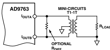
Figure 16. Differential Output Using a Transformer
