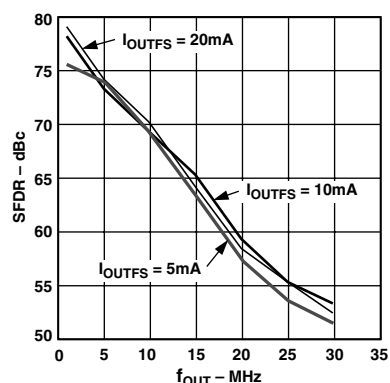
TPC 6. SFDR vs. f_{OUT} and I_{OUTFS} @ 65 MSPS and 0 dBFS
