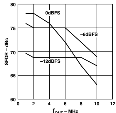
TPC 3. SFDR vs. f_{OUT} @ 25 MSPS
