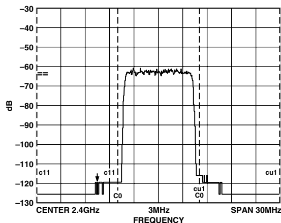
Figure 25. CDMA Signal, 8 M Chips Sampled at 65 MSPS, Recreated at 2.4 GHz, Adjacent Channel Power &gt; 60 dBm
