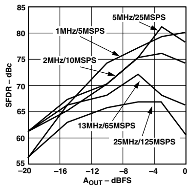
TPC 8. Single-Tone SFDR vs. A_{OUT} @ f_{OUT} = f_{CLOCK}/5
