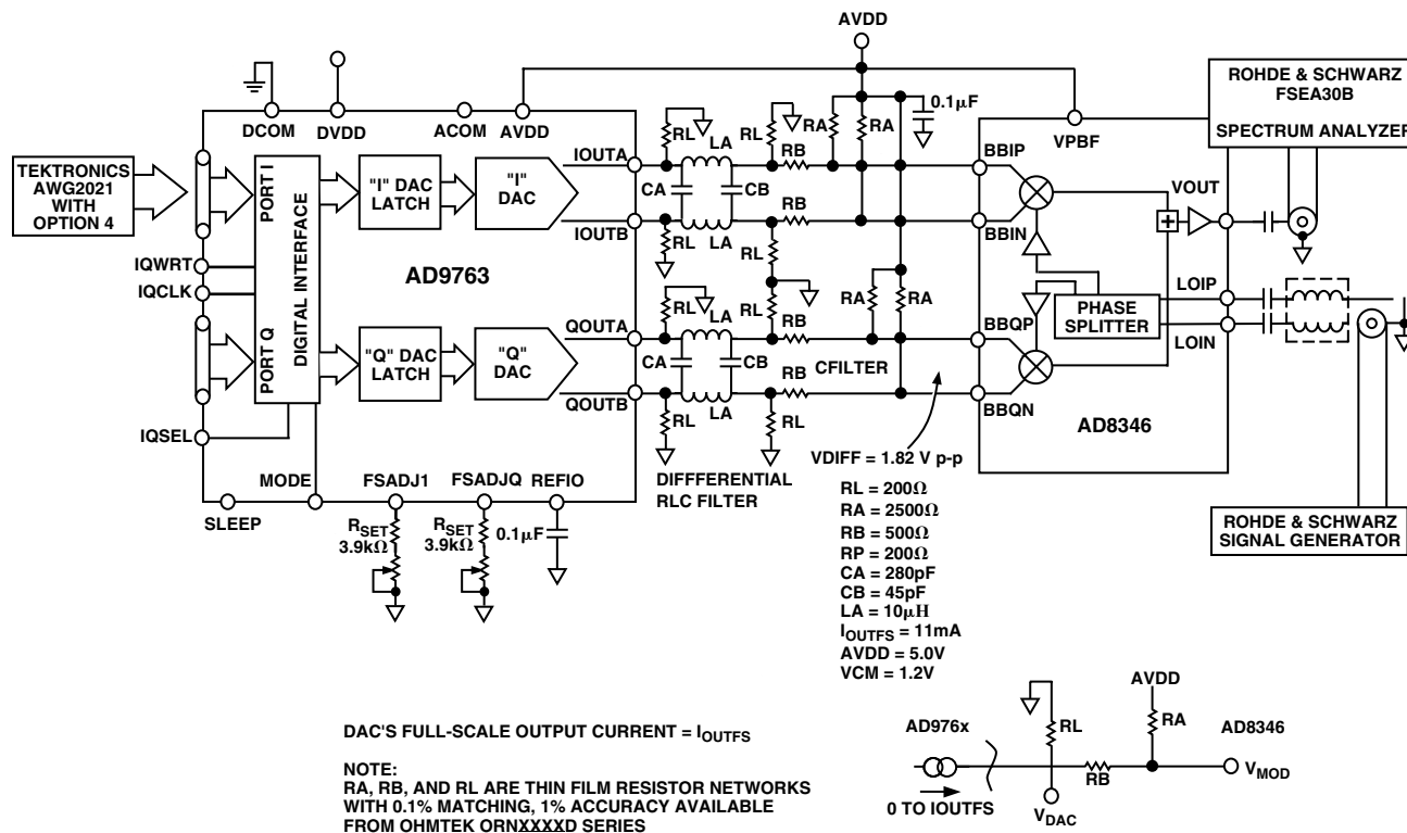
Figure 24. Baseband QAM Implementation Using an AD9763 and AD8346
