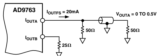
Figure 19. 0 V to 0.5 V Unbuffered Voltage Output
