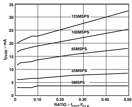
Figure 14. I_{DVDD} vs. Ratio @ DVDD = 5 V
