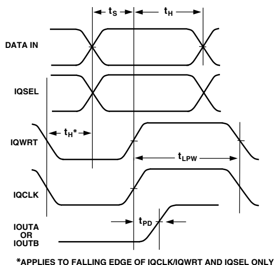
Figure 9. Interleaved Mode Timing
