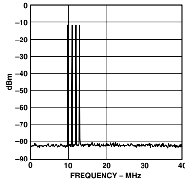
TPC 17. Four-Tone SFDR @ f_{\text{CLK}} = 125 \text{ MSPS}
