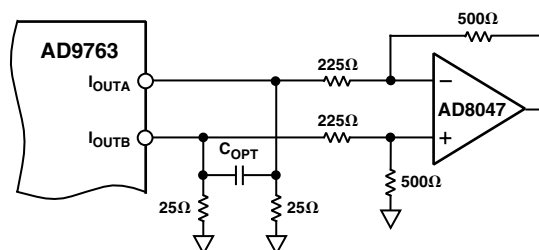
Figure 17. DC Differential Coupling Using an Op Amp
