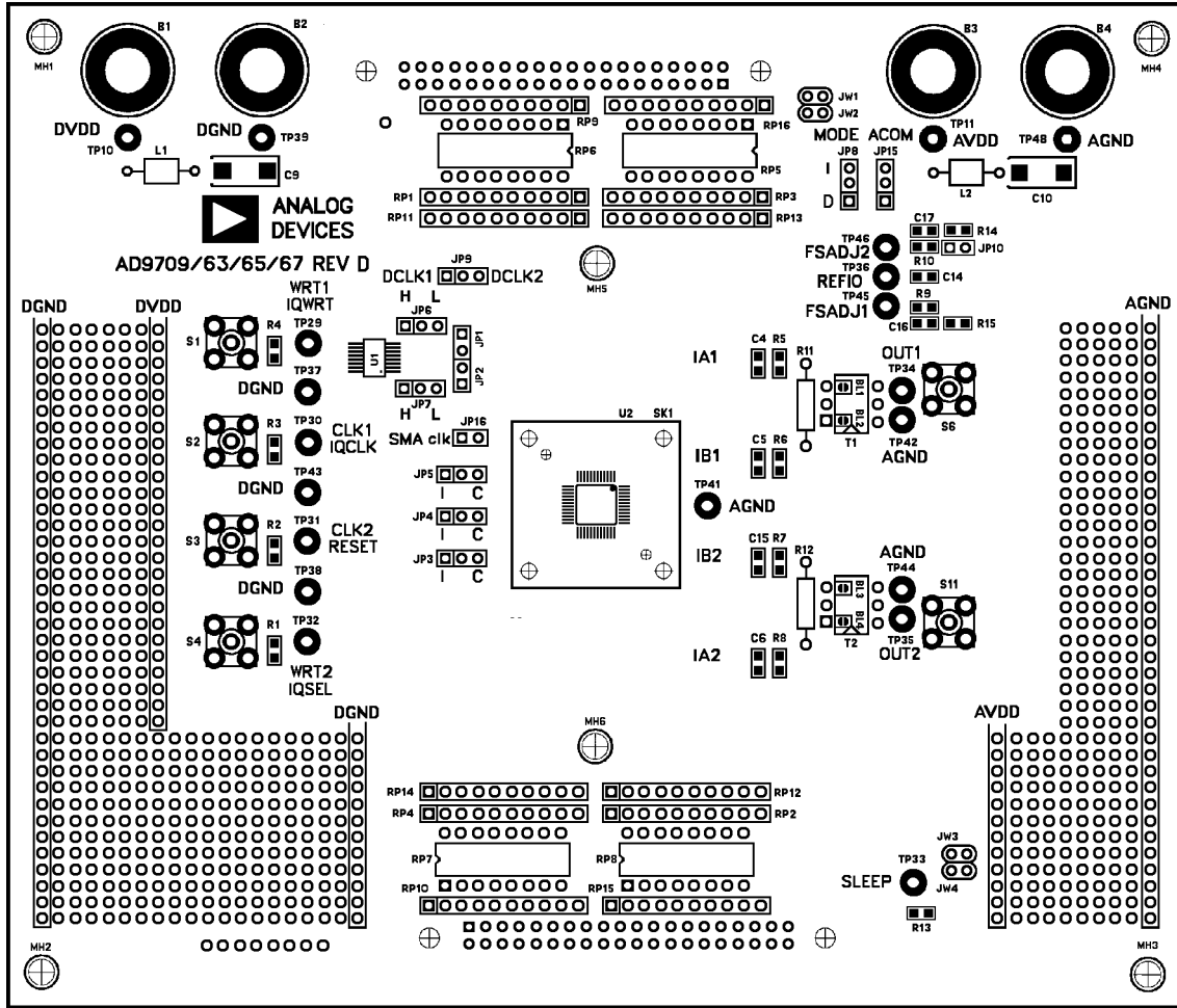
Figure 30. Assembly, Top Side
