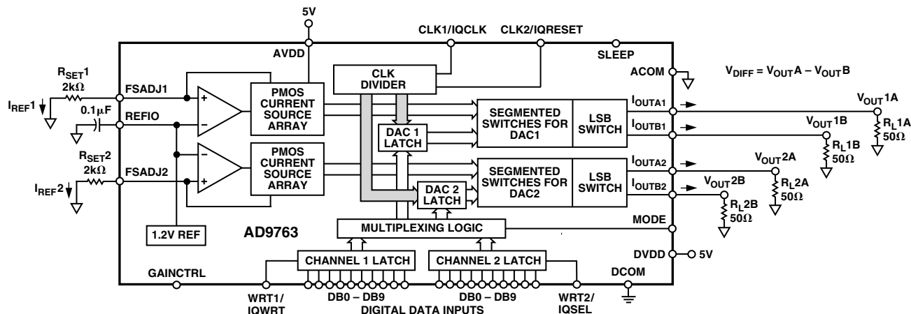
Figure 3. Simplified Block Diagram
