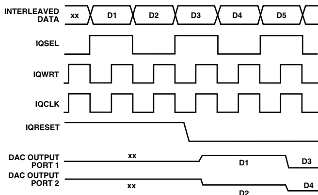
Figure 10. Interleaved Mode Timing
