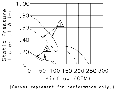
Performance Curve: 6 in. Fans
