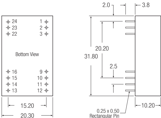
DIP24 Package Style
