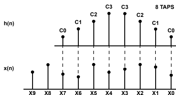
FIGURE 6. DATA/COEFFICIENT ALIGNMENT FOR 8-TAP EVEN SYMMETRIC FILTER
