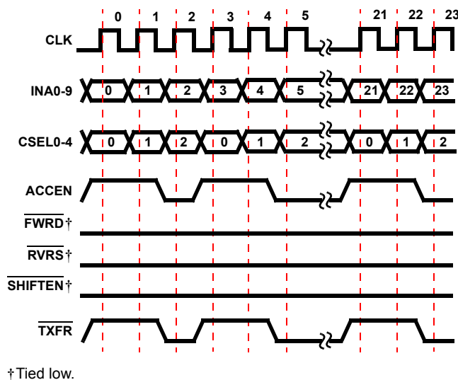
FIGURE 18. CONTROL SIGNAL TIMING FOR 24-TAP DECIMATE X3 FILTER
