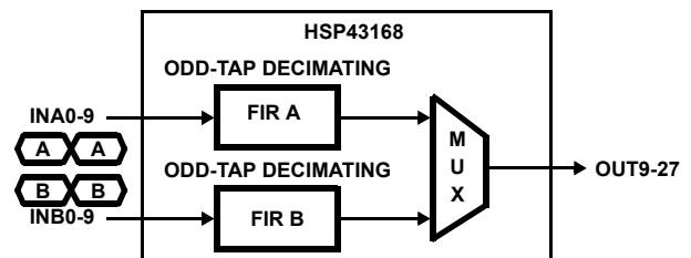
FIGURE 19. USING HSP43168 AS TWO INDEPENDENT FILTERS
