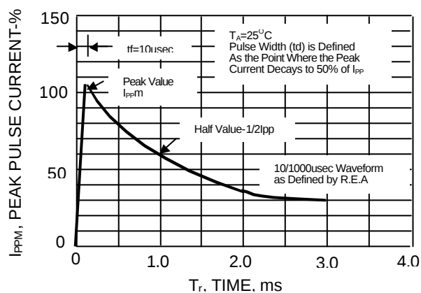
Fig. 3-PULSE WAVEFORM
