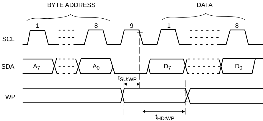
Figure 9. WP Timing
