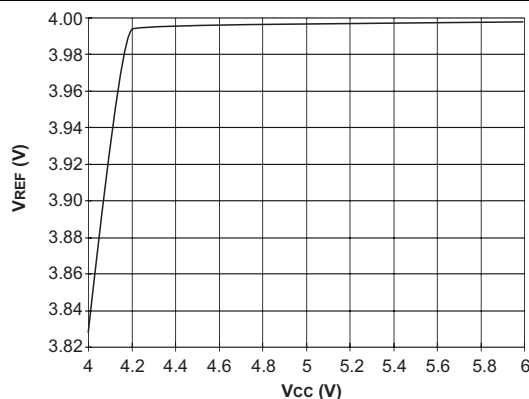
Figure 6-2. UCC2803 and UCC2805 V_{REF} vs V_{CC} , I_{LOAD} = 0.5 mA
