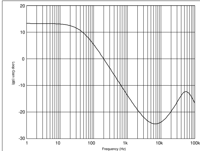
Figure 8-2. Converter Open Loop Bode Plot - Gain
