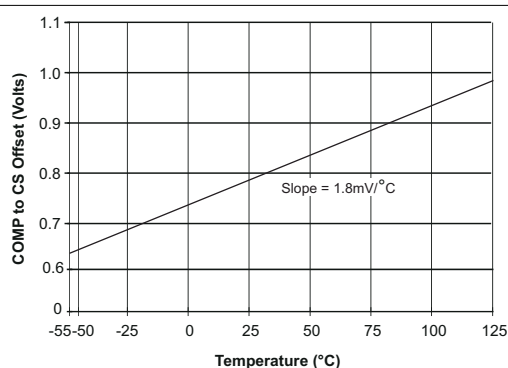
Figure 6-10. COMP to CS Offset vs Temperature, CS = 0 V
