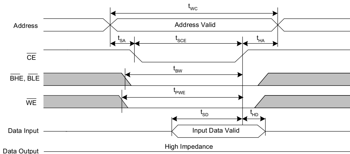
Figure 11. SRAM Write Cycle No. 2 ( \overline{\text{CE}} Controlled) [36, 37, 38, 39]
