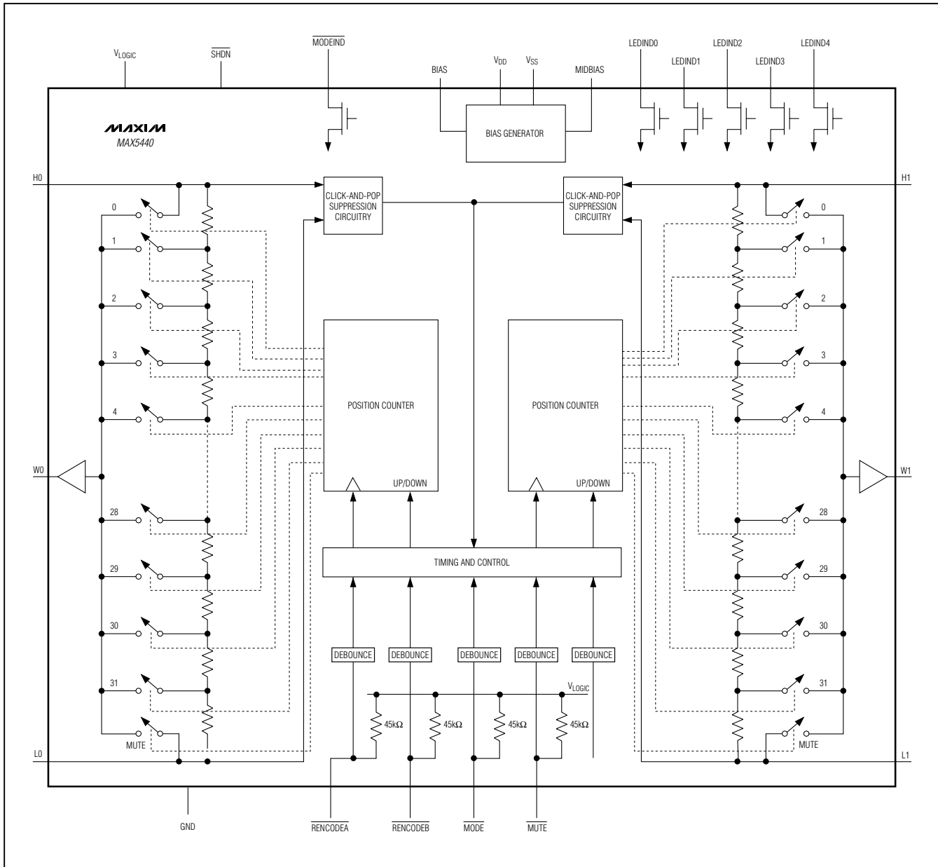
Functional Diagram
