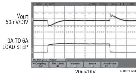
1.2V Transient Response
