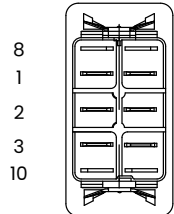
BOTTOM VIEW TERMINAL ARRANGEMENT 10 TERMINAL BASE
