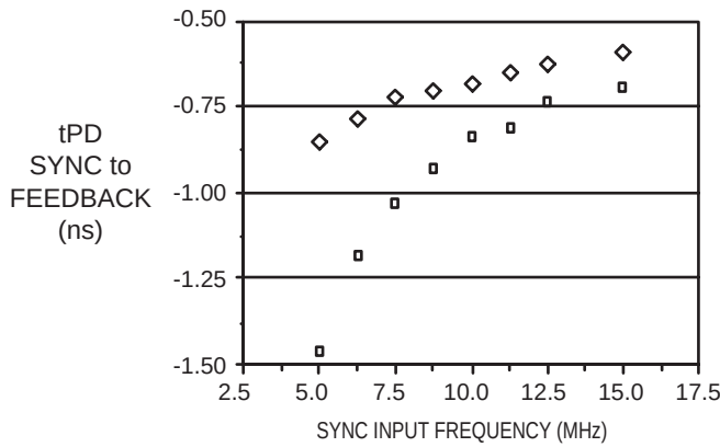
tPD versus Frequency for Q/2 output feed back, including process and voltage variation at 25°C (with 1 MΩ resistor tied to analog VCC)
