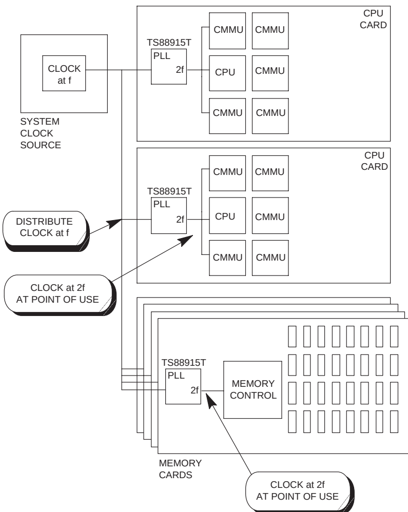
Figure 12. Representation of a Potential Multi-Processing Application Utilizing the TS88915T for Frequency Multiplication and Low Board-to-board Skew
