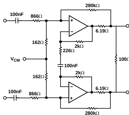
Figure 32. ADSL/ADSL2+ Circuit
