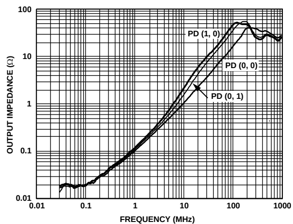
Figure 31. Output Impedance vs. Frequency Quad Op Amp Circuit (Figure 29) V_S = \pm 12\text{ V} , G = +5 , PD(0, 0)
