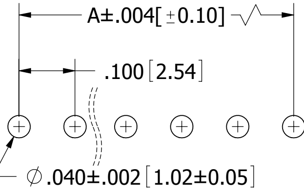
RECOMMENDED PCB LAYOUT SINGLE ROW TOLERANCE: ± .002 [ ± 0.05 ]
