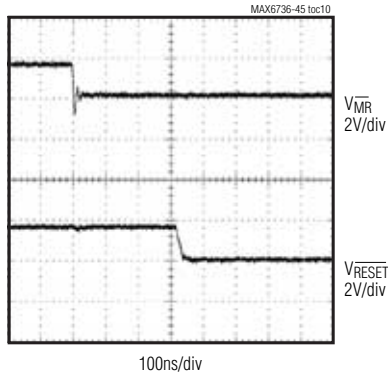
\overline{\text{MR}} TO RESET OUTPUT DELAY
