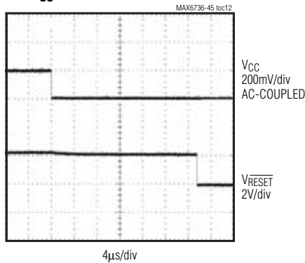
V_{\text{CC}} TO RESET OUTPUT DELAY
