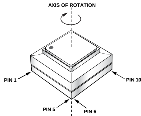
Figure 4. Pin Configuration
