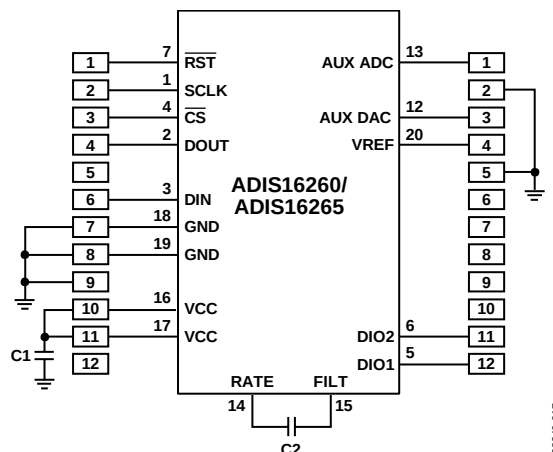
Figure 19. Electrical Schematic
