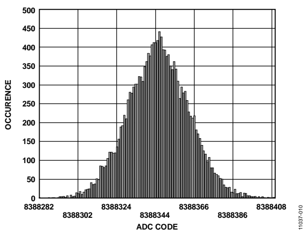
Figure 10. Noise Distribution Histogram ( AVDD1 = 5\text{ V} , AVDD2 = 5\text{ V} , V_{REF} = 5\text{ V} , IOVDD = 3.3\text{ V} , Output Data Rate = 250 kSPS)
