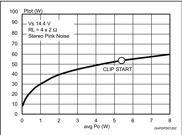
Figure 24. Power dissipation vs. average Po (audio program simulation, 2 \Omega )
