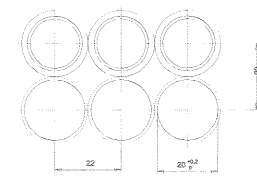
panel cutout
