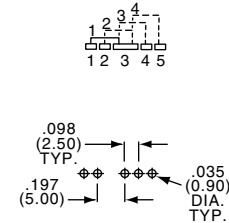
P. C. HOLE LAYOUT
