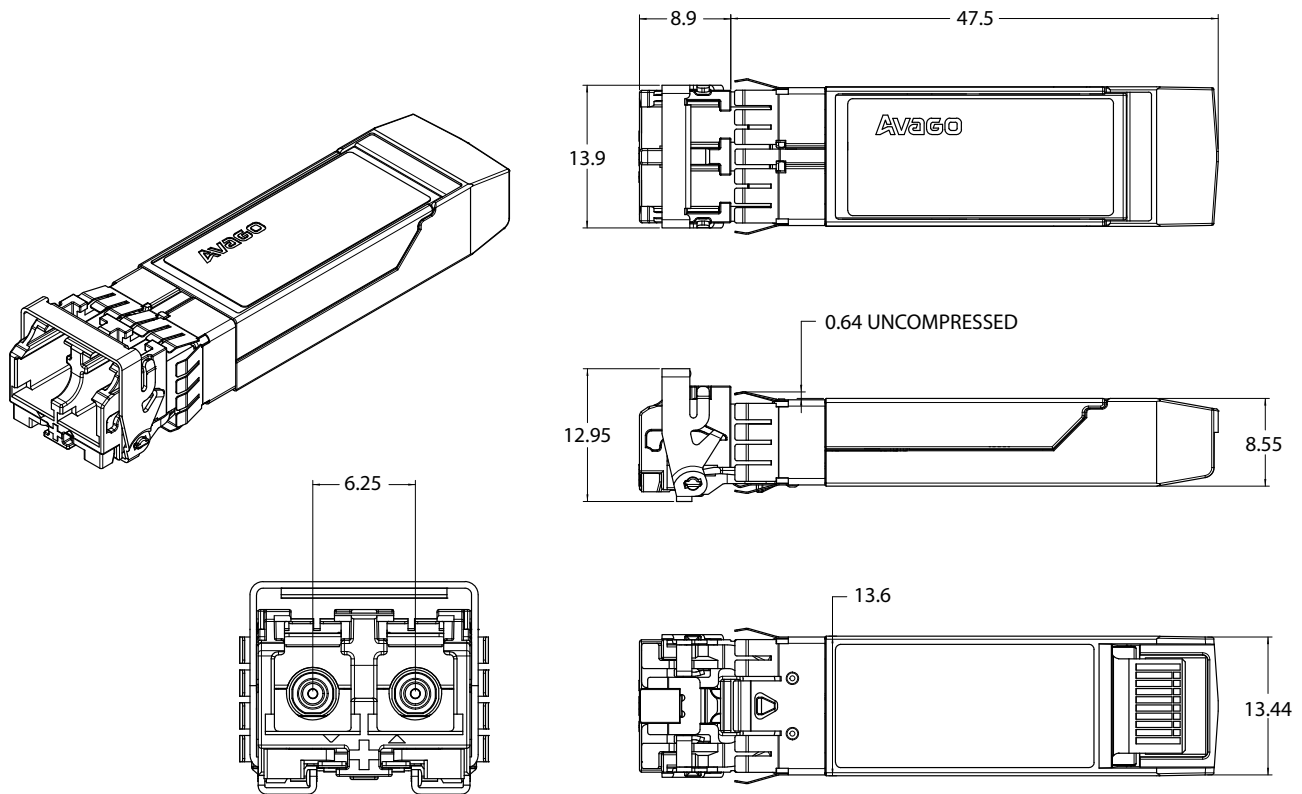
Figure 7. Module drawing
