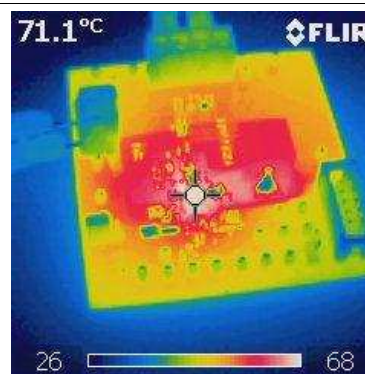
Natural Convection
