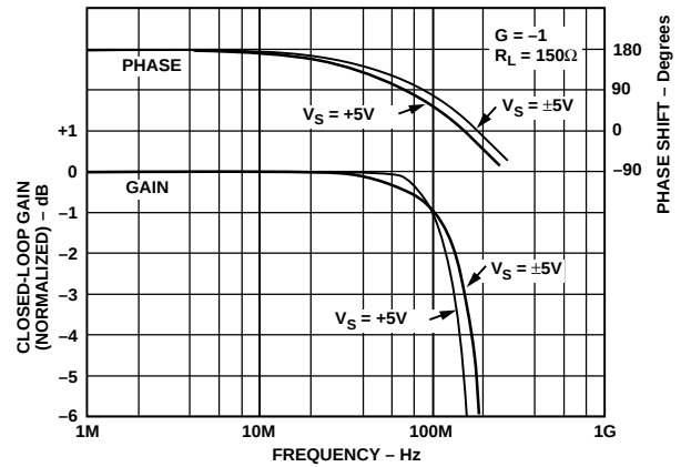
Figure 25. Closed-Loop Gain and Phase vs. Frequency, G = -1 , R_L = 150 \Omega
