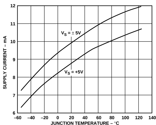
Figure 4. Total Supply Current vs. Junction Temperature
