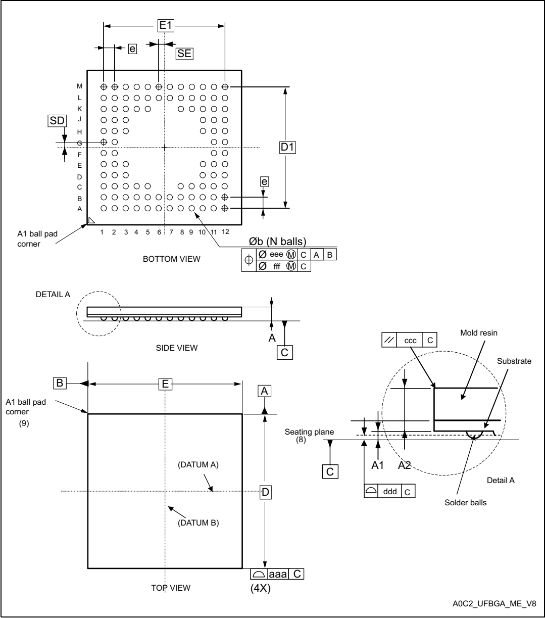
Figure 71. UFBGA100 - Outline (13)
