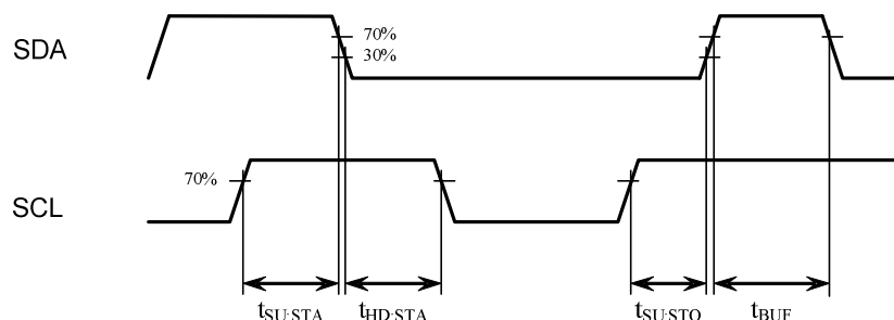
Figure 6 I2C Start and Stop timing
