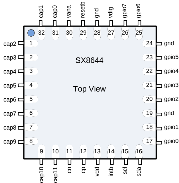
Figure 3 Pinout Diagram LQFP
