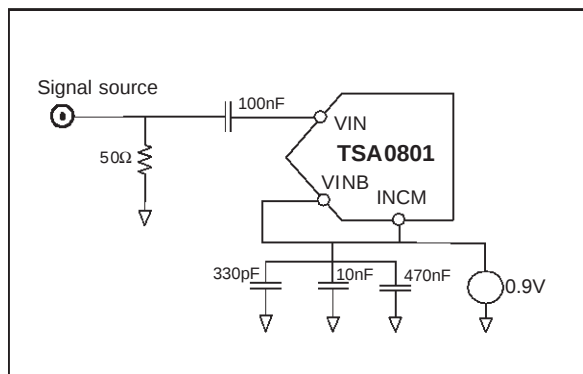
Figure 6 : Single-ended input configuration
