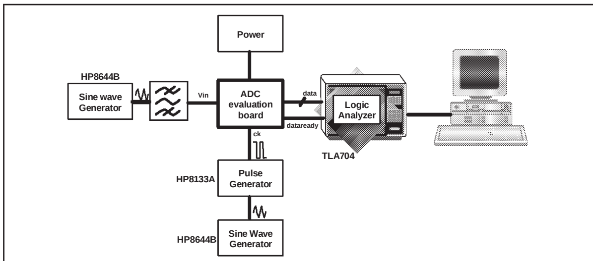
Figure 9 : Analog to Digital Converter characterization bench
