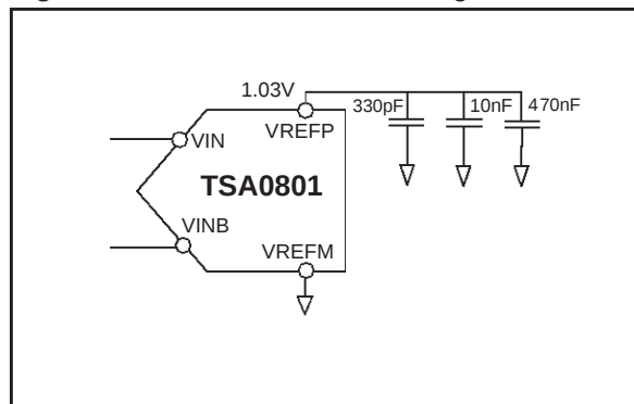
Figure 7 : Internal reference setting
