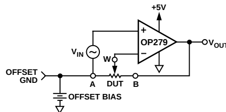
Figure 27. Noninverting Programmable Gain Test Circuit
