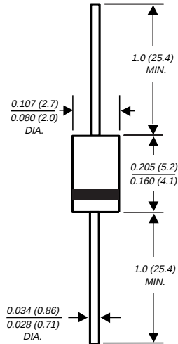
DO-204AL
