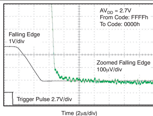
Figure 69. Full-Scale Settling Time 2.7 V Falling Edge
