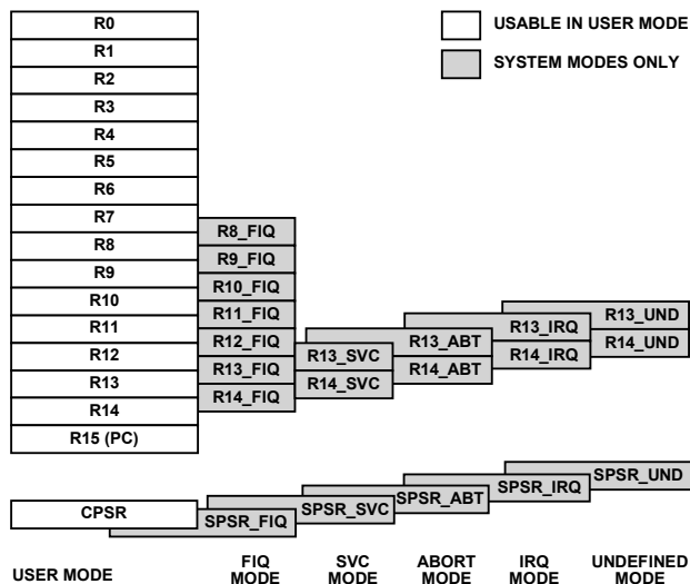
Figure 15. Register Organization
