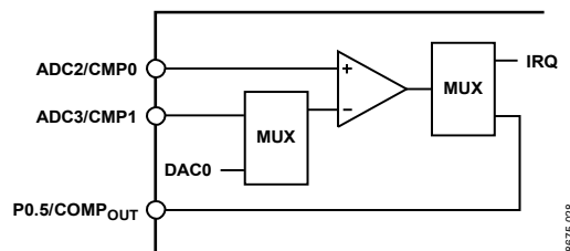
Figure 34. Comparator
