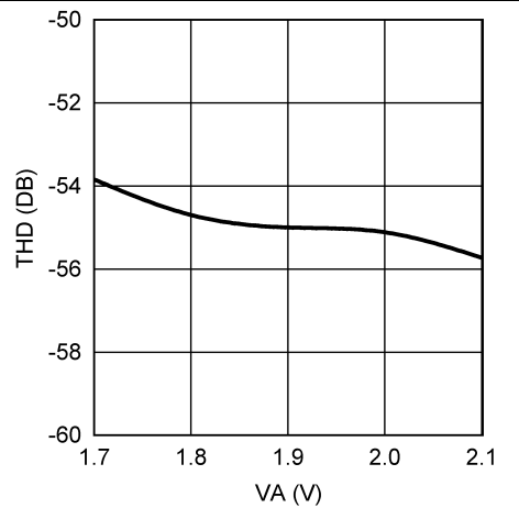
Figure 27. THD vs. SUPPLY VOLTAGE
