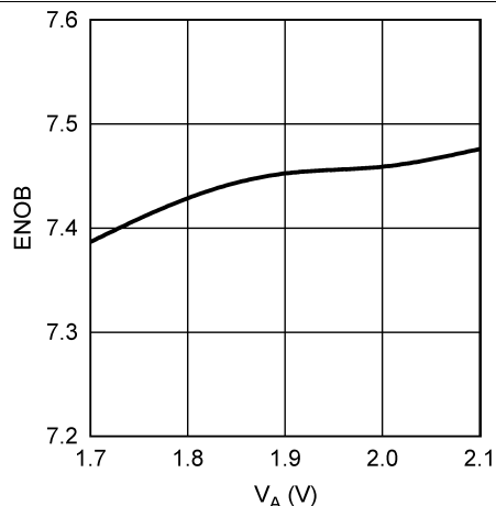
Figure 19. ENOB vs. SUPPLY VOLTAGE
