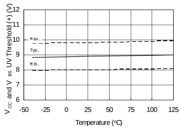
Figure 21. V CC and V BS Undervoltage Threshold (+) vs. Temperature
