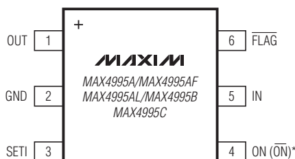
SOT23 (1.6mm × 2.9mm)
