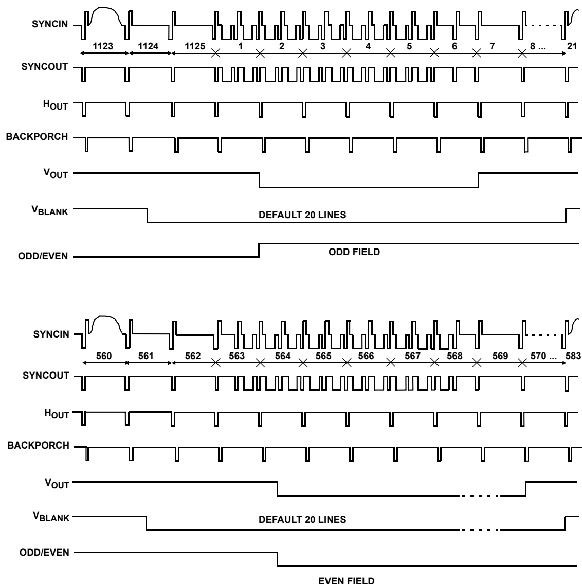
FIGURE 6. EXAMPLE OF HDTV 1080I/30 LINE COMPOSITE VIDEO: INTERLACED, ODD &amp; EVEN FIELD
