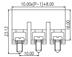
Dimensions - mm
