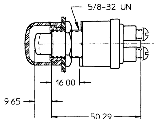
9245 dimensions
