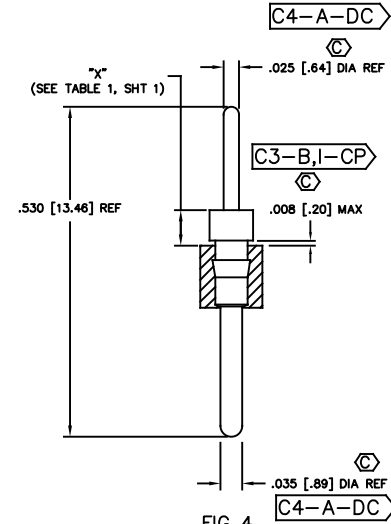
FIG 4 TERMINAL STYLE -A-2 T-1R7-2-X
