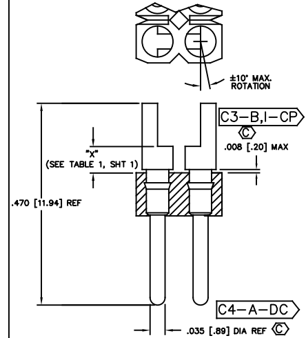
FIG 10 TERMINAL STYLE -C-2 T-1R9-2-X
