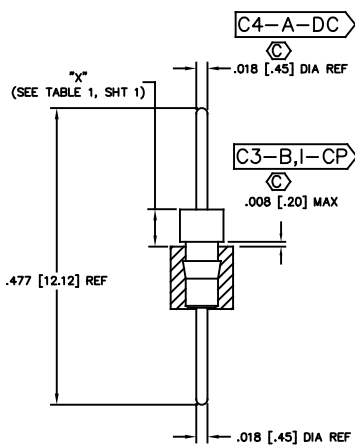
FIG 1 TERMINAL STYLE -AA T-1R5-X
