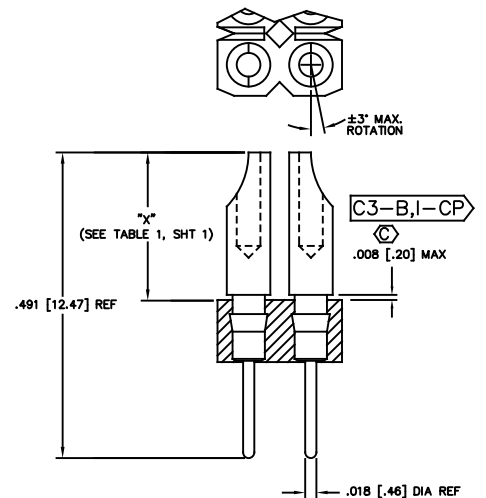
FIG 5 TERMINAL STYLE -B T-1R1-X
