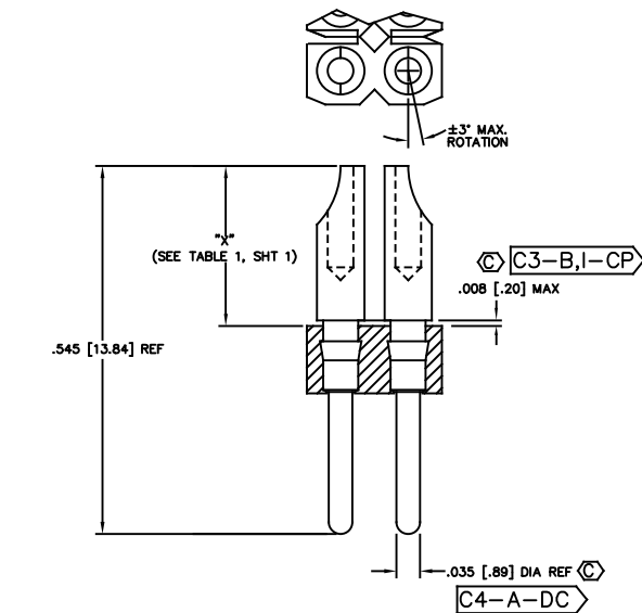
FIG 7 TERMINAL STYLE -B-2 T-1R8-2-X
