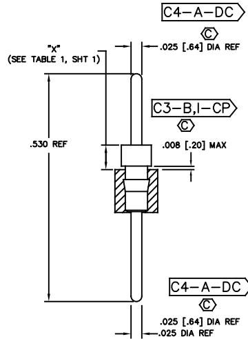
FIG 3 TERMINAL STYLE -A-1 T-1R7-1-X
