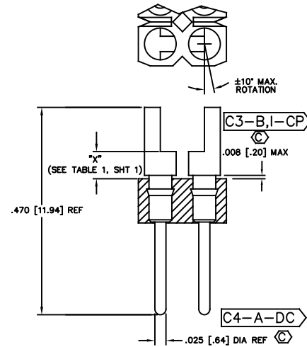
FIG 9 TERMINAL STYLE -C-1 T-1R9-1-X
