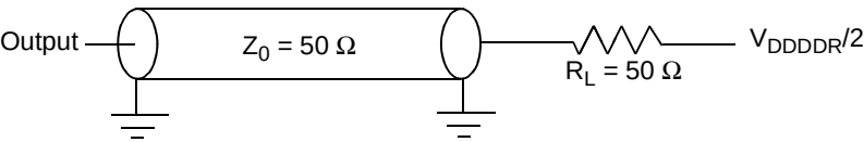
Figure 10. DDR AC Test Load
