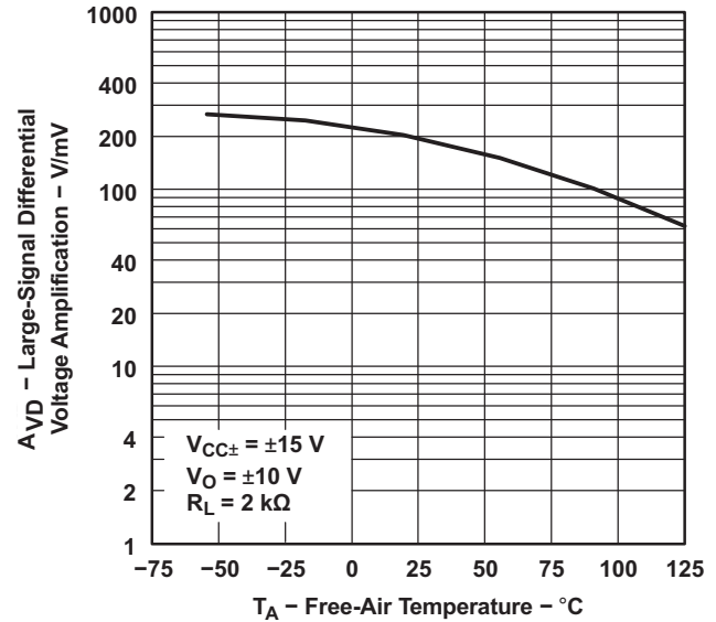
Figure 11. Large-Signal Differential Voltage Amplification vs Free-Air Temperature
