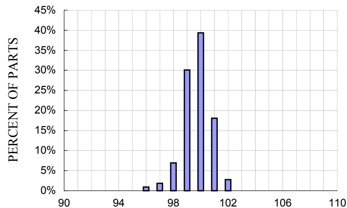
mV/g X-axis Sensitivity Distribution at Xout, V DD =5V
