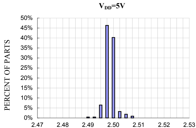
Voltages X-axis Zero g Bias Distribution at Xout, V DD =5V
