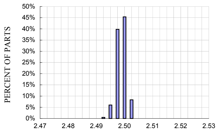
Voltages Y-axis Zero g Bias Distribution at Yout, V DD =5V
