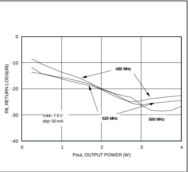
Figure 8. Return loss vs. output power
