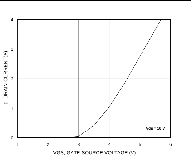
Figure 3. Drain current vs. gate voltage
