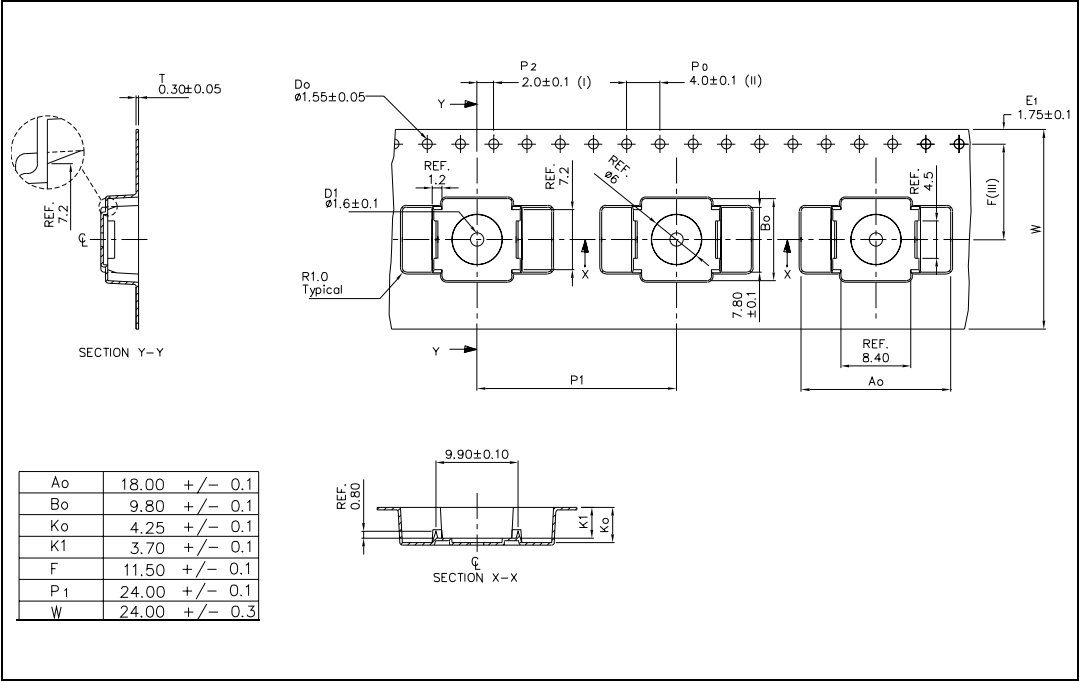
Figure 29. Reel information
