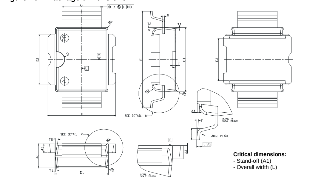
Figure 26. Package dimensions
