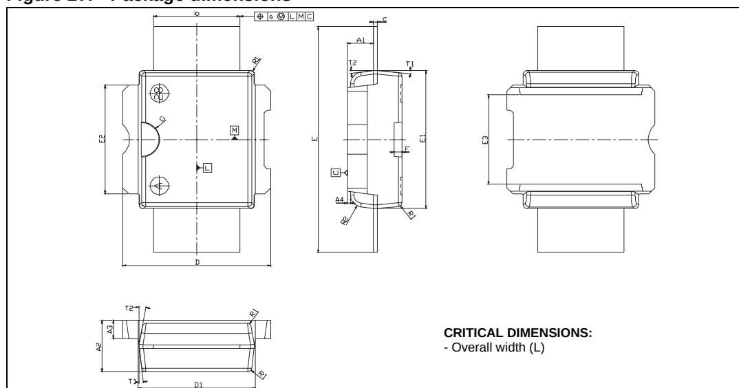
Figure 27. Package dimensions
