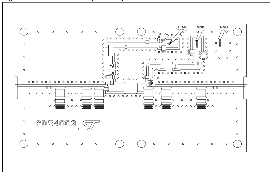
Figure 25. Test circuit photomaster
