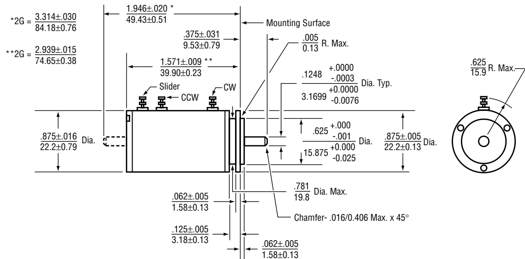
Model 7223 Servo Mount with Ball Bearing
