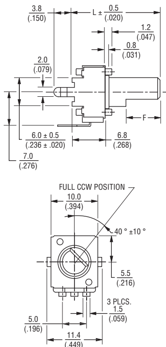
PTV09A-4 (Horizontal/Rear Mount, Bushingless)
