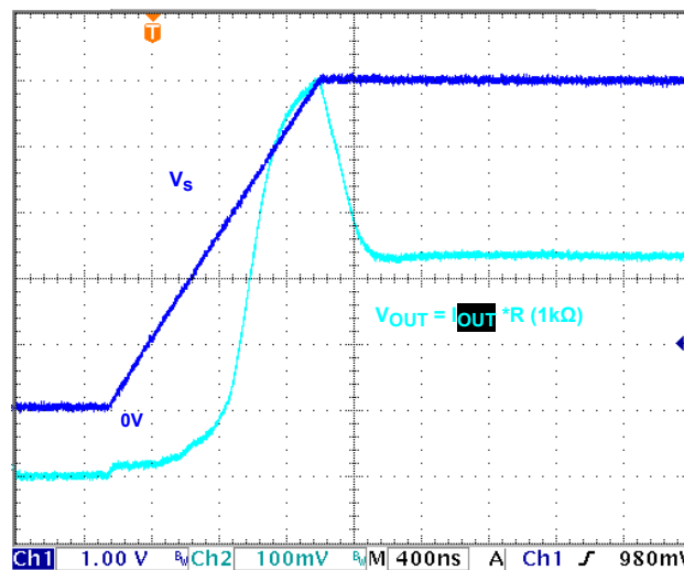
FIGURE 17. V_S RAMP = 5V/ \mu s, I_{OUT} TURN-ON
