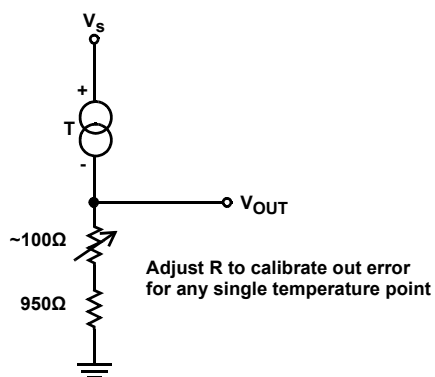
FIGURE 14. SINGLE TEMPERATURE ERROR CALIBRATION
