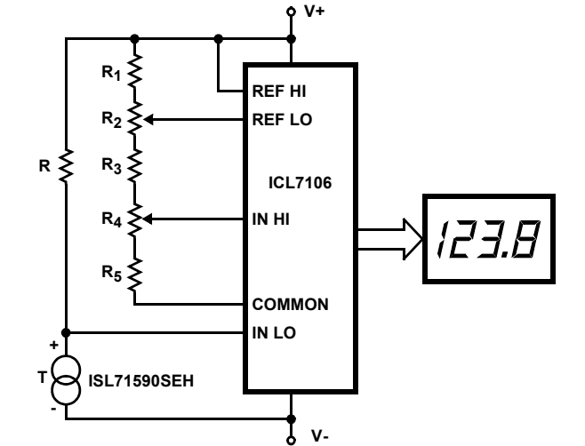
FIGURE 34. BASIC DIGITAL THERMOMETER, CELSIUS, AND FAHRENHEIT SCALES
