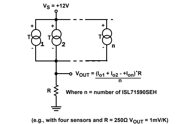
FIGURE 31. AVERAGE TEMPERATURE SENSING SCHEME
