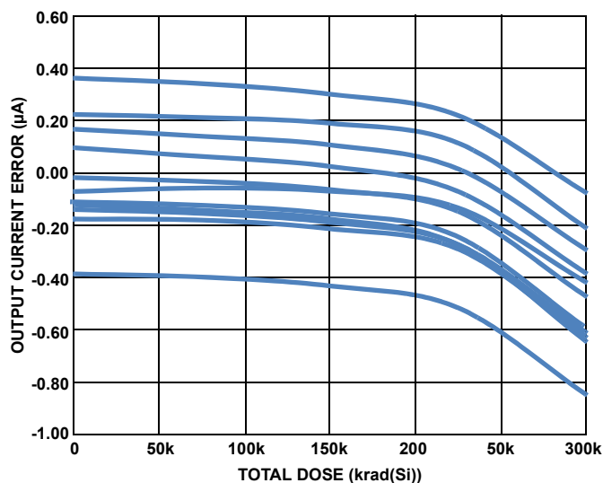
FIGURE 19. TYPICAL ABSOLUTE I_{OUT} ERROR vs TOTAL IONIZING DOSE FOR HIGH DOSE RATE (ISL71590SEH ONLY)
