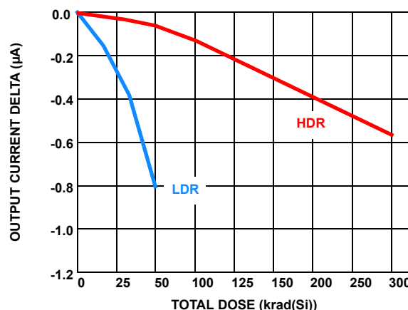
FIGURE 2. I_{\text{OUT}} SHIFT vs LOW/HIGH DOSE RATE RADIATION
