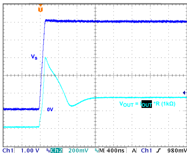
FIGURE 18. V_S RAMP = 50V/ \mu s, I_{OUT} TURN-ON
