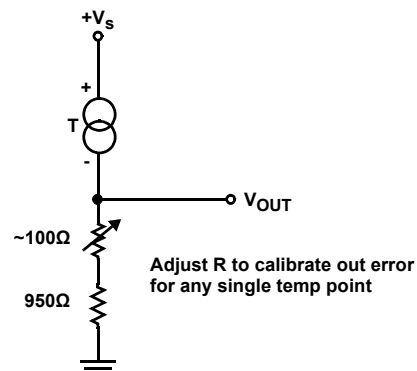
FIGURE 21. SLOPE TRIMMING
