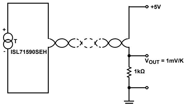
FIGURE 28. TYPICAL APPLICATION
