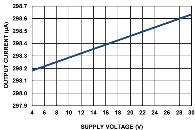
FIGURE 7. OUTPUT CURRENT vs V_S VOLTAGE
