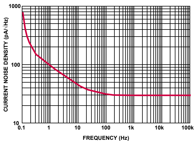
FIGURE 11. CURRENT NOISE DENSITY vs FREQUENCY
