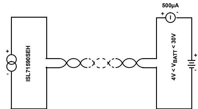
FIGURE 33. SIMPLEST THERMOMETER
