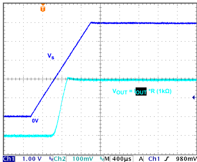
FIGURE 16. V_S RAMP = 3.7V/ms, I_{OUT} TURN-ON
