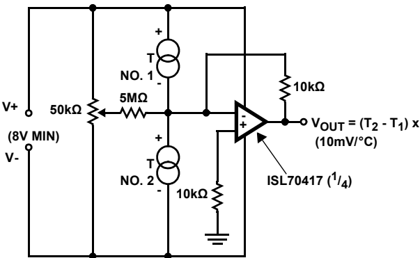
FIGURE 38. DIFFERENTIAL THERMOMETER
