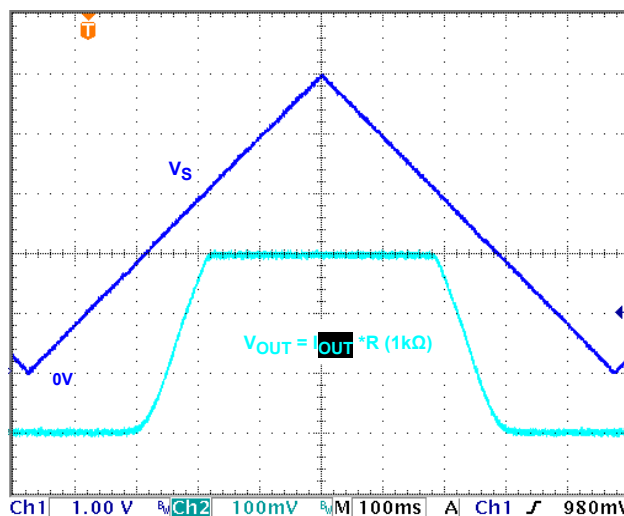
FIGURE 15. TURN-ON/OFF V_S VOLTAGE
