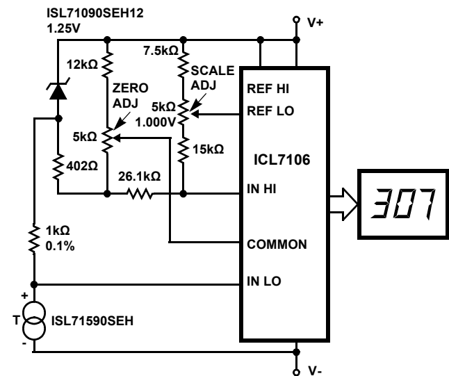
FIGURE 36. BASIC DIGITAL THERMOMETER, KELVIN SCALE WITH ZERO ADJUST
