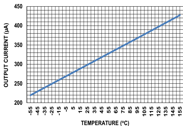
FIGURE 6. OUTPUT CURRENT vs TEMPERATURE
