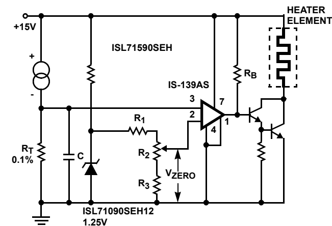
FIGURE 32. SINGLE SETPOINT TEMPERATURE CONTROLLER
