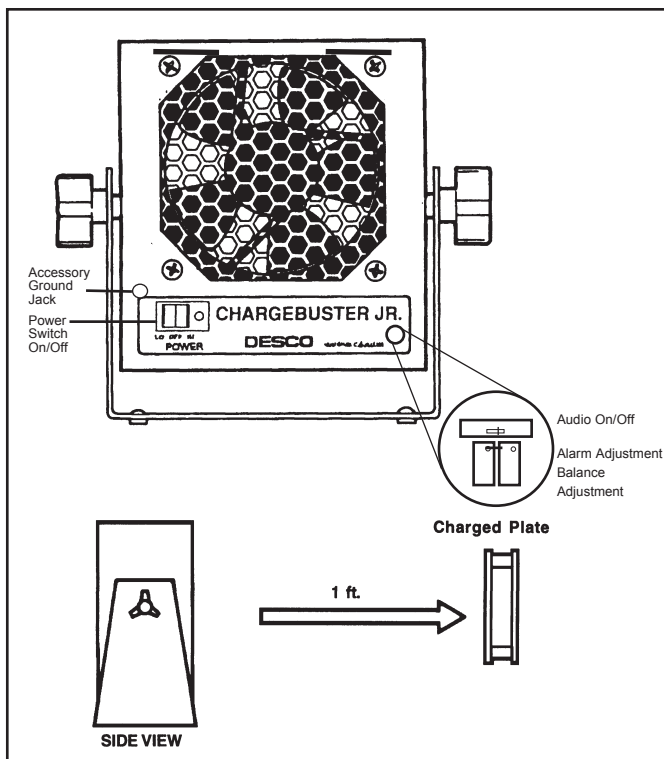
Figure 8. Calibration and position of charged plate for calibration.
