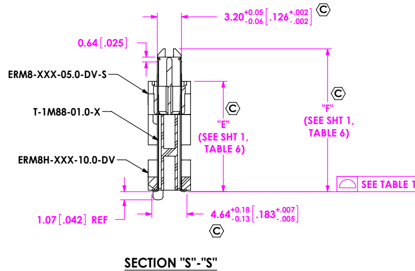
FIG 7 (**ERM8-030-T5.0-X-DV SHOWN) (SOME CENTER FEATURES REMOVED FOR CLARITY) ***NOT TOOLED
