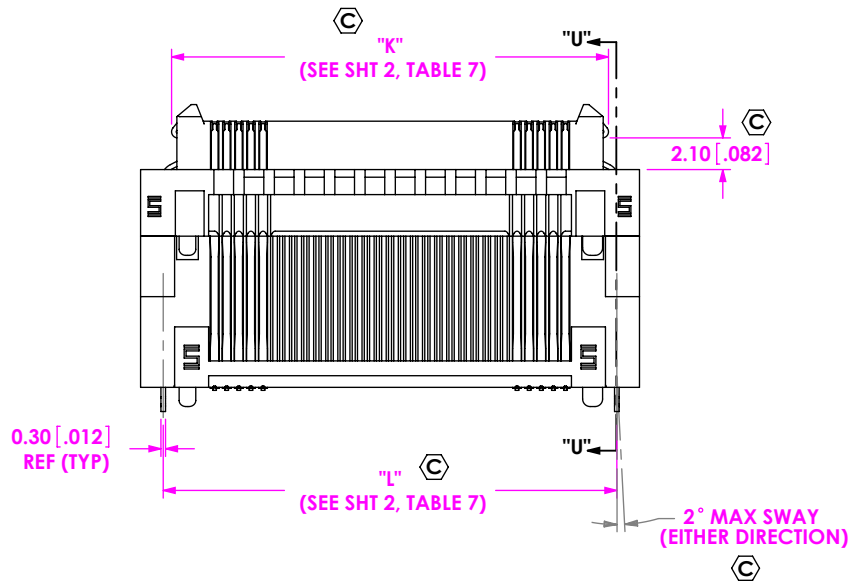
FIG 8 (**ERM8-030-T5.0-X-DV-L SHOWN) (SAME AS FIG. 7, EXCEPT AS SHOWN) ***NOT TOOLED
