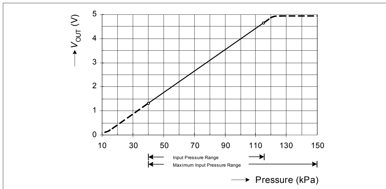
Figure 3 Transfer Function
