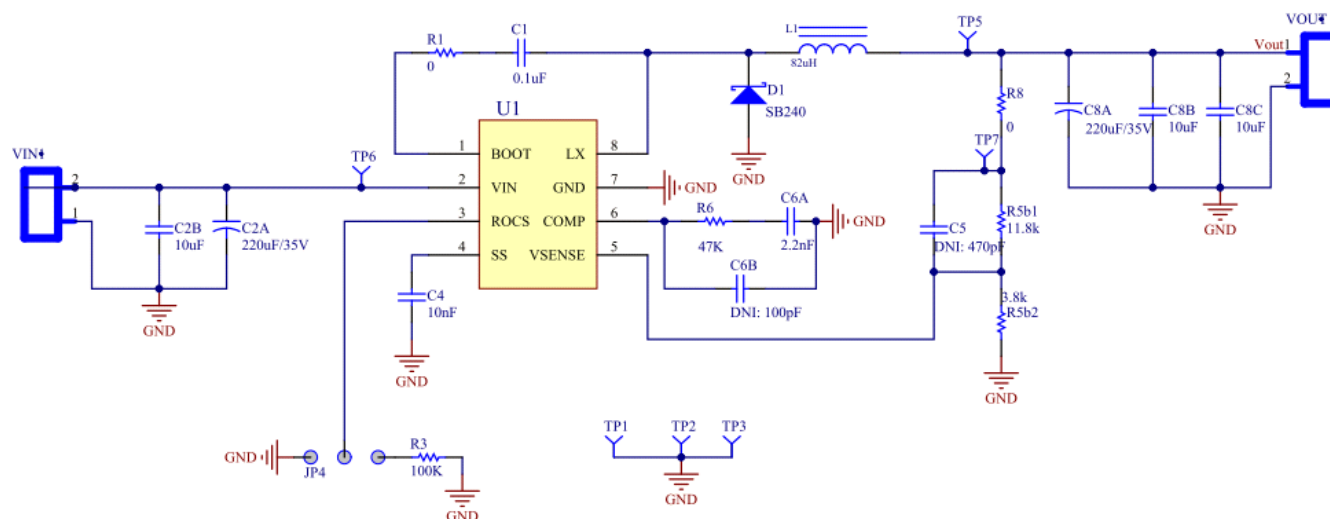
Figure 6-1. TPS5402EVM Schematic
