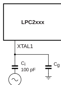
Fig 22. Slave mode operation of the on-chip oscillator
